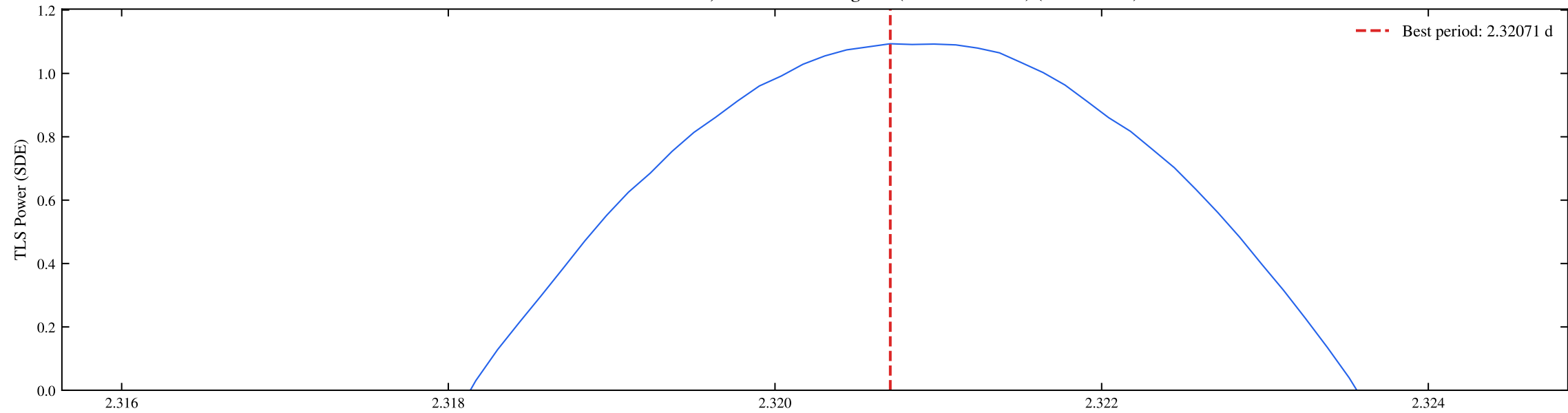
TIC 117789567 | Sectors: 54, 55 | TLS Periodogram (Planet 2 Search) (SDE = 7.96)
