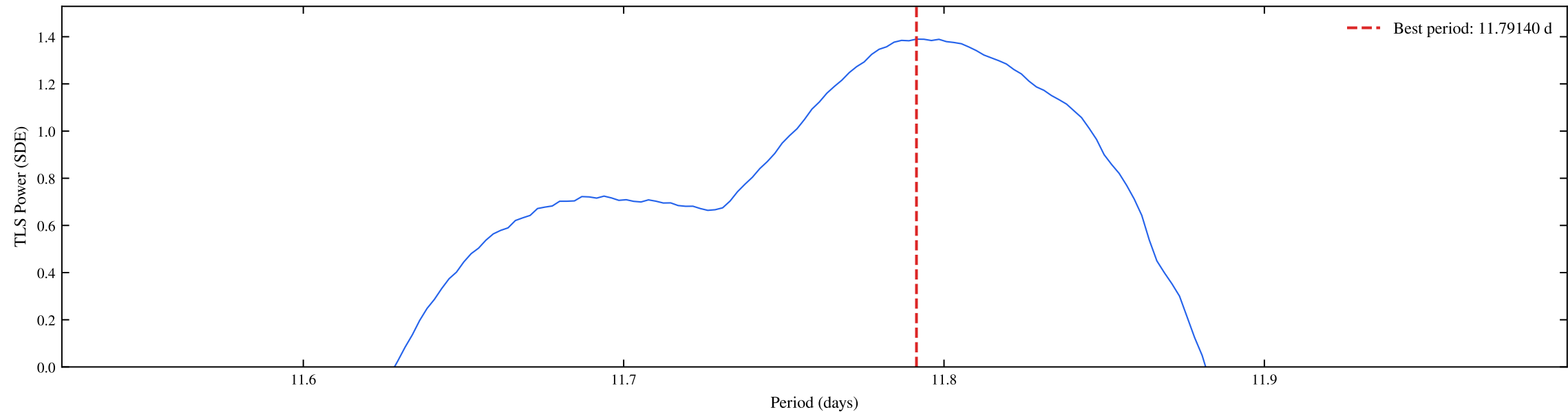
TIC 117789567 | Sectors: 54, 55 | TLS Fine Periodogram (SDE = 1.39)
