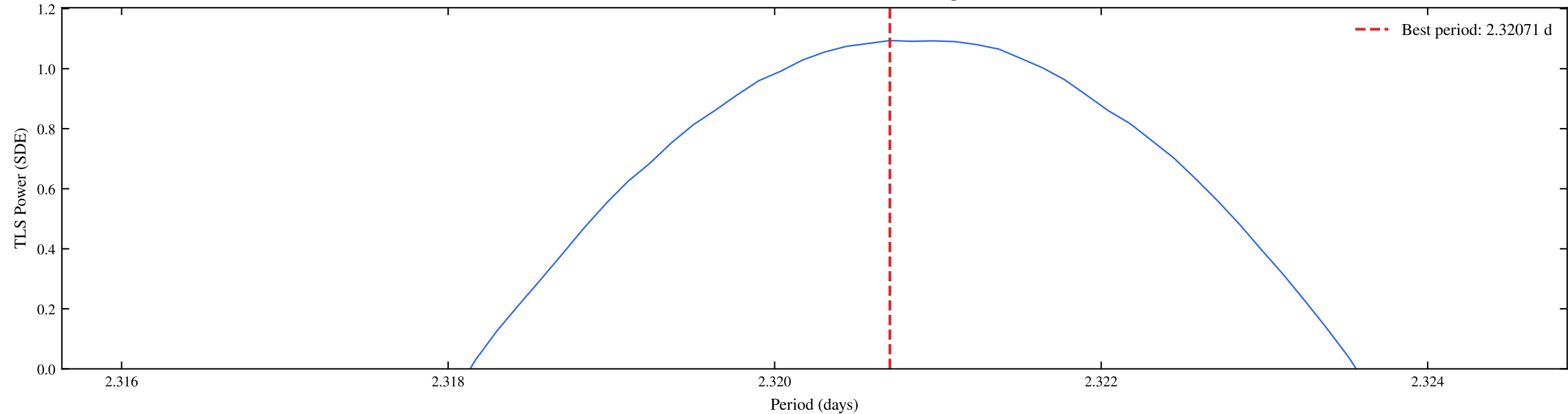
TIC 117789567 | Sectors: 54, 55 | TLS Coarse Periodogram (SDE = 1.09)
