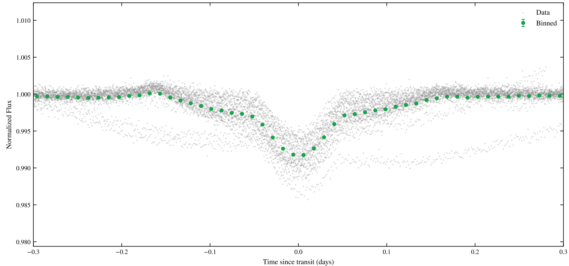
TIC 117789567 | Sectors: 54, 55 | Phase-Folded Transit ( P = 2.32071 d)
