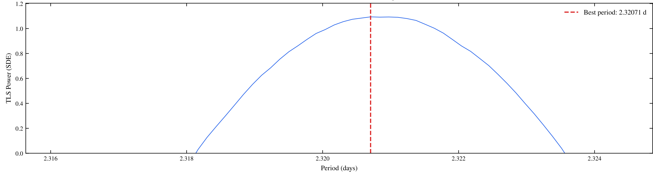
TIC 117789567 | Sectors: 54, 55 | TLS Fine Periodogram (SDE = 1.09)
