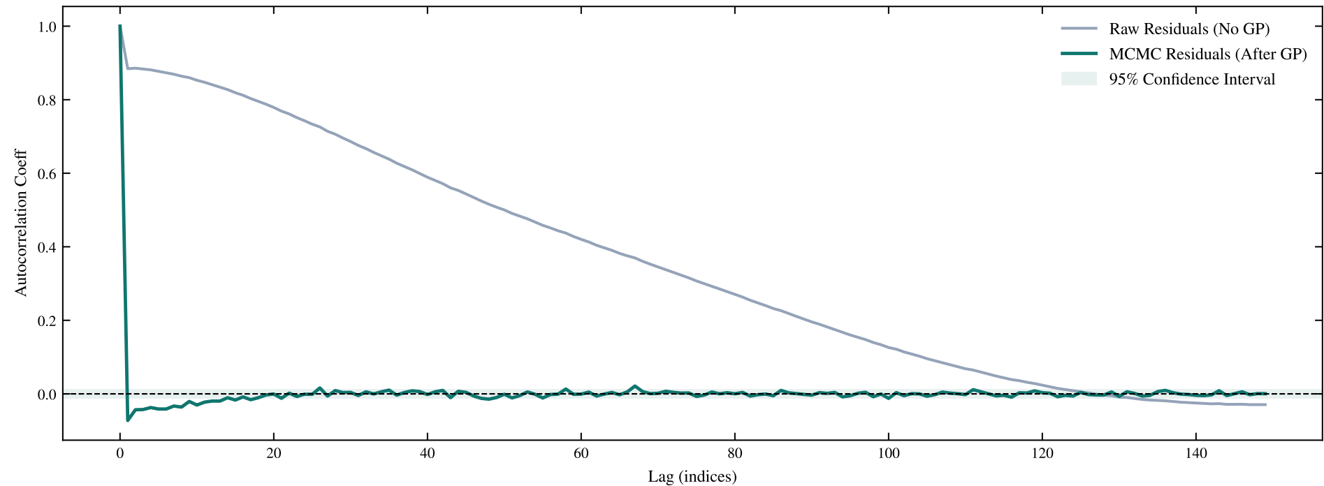
TIC 117789567 | Sectors: 54, 55 | GP Residuals Autocorrelation Function (ACF)
