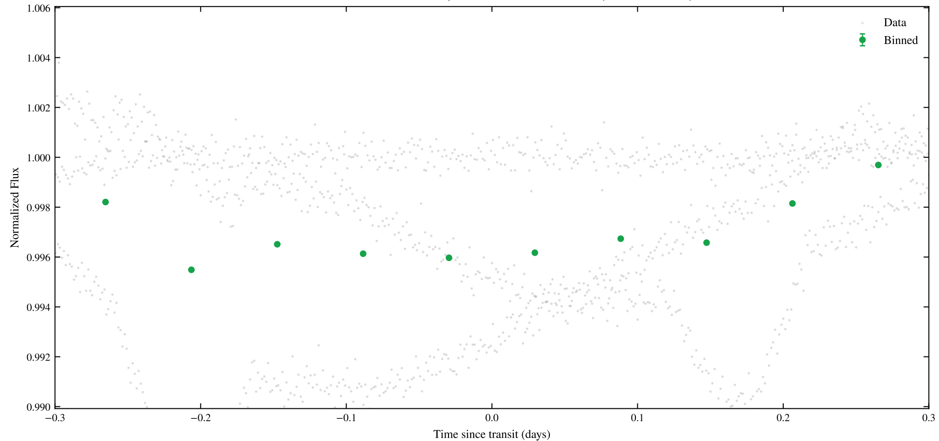
TIC 117789567 | Sectors: 54, 55 | Phase-Folded Transit (P = 11.79140 d)
