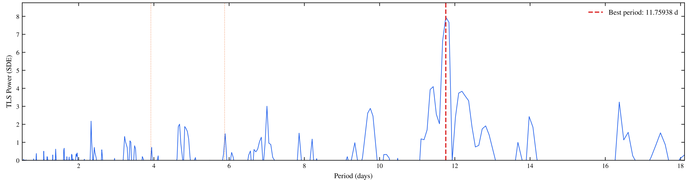
TIC 117789567 | Sectors: 54, 55 | TLS Coarse Periodogram (SDE = 7.96)
