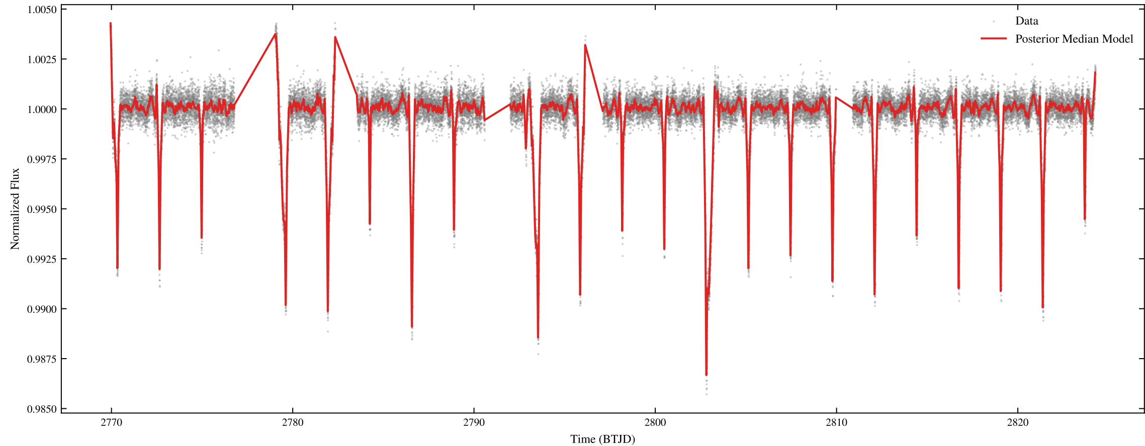
TIC 117789567 | Sectors: 54, 55 | MCMC Posterior Predictive Check
