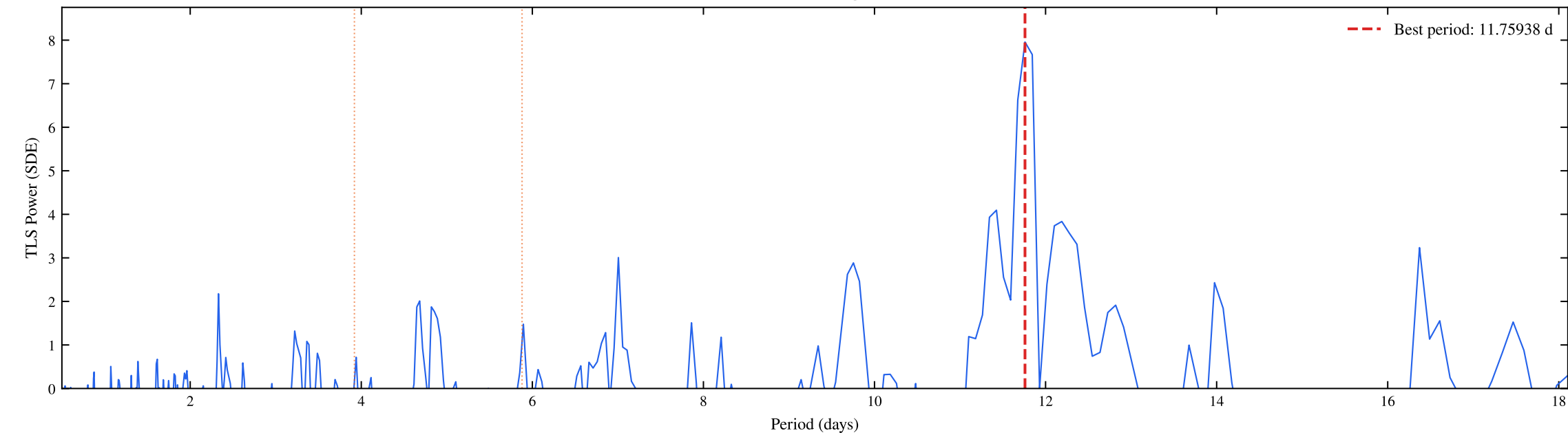
TIC 117789567 | Sectors: 54, 55 | TLS Periodogram (Planet 2 Search) (SDE = 7.96)
